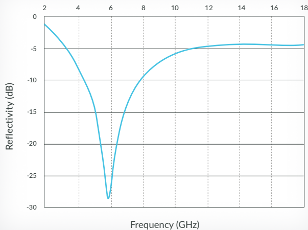
REFLECTIVITY PERFORMANCE
