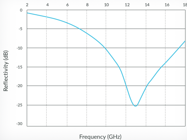
REFLECTIVITY PERFORMANCE
